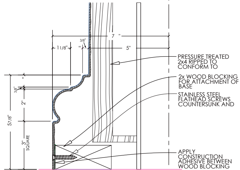
SECTION @ COLUMN BASE
