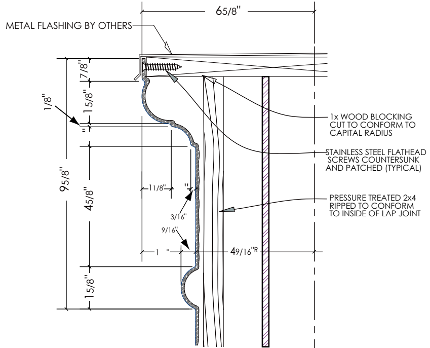
SECTION @ COLUMN CAPITAL
