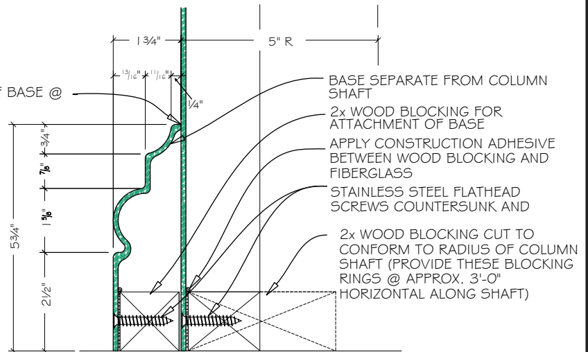
SECTION @ COLUMN BASE
