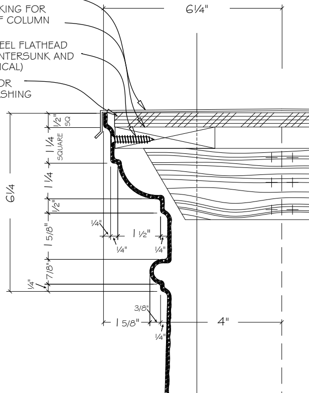
SECTION @ COLUMN CAPITAL
