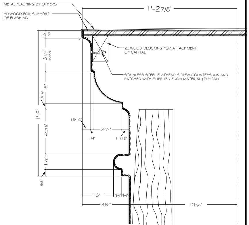
SECTION @ COLUMN CAPITAL
