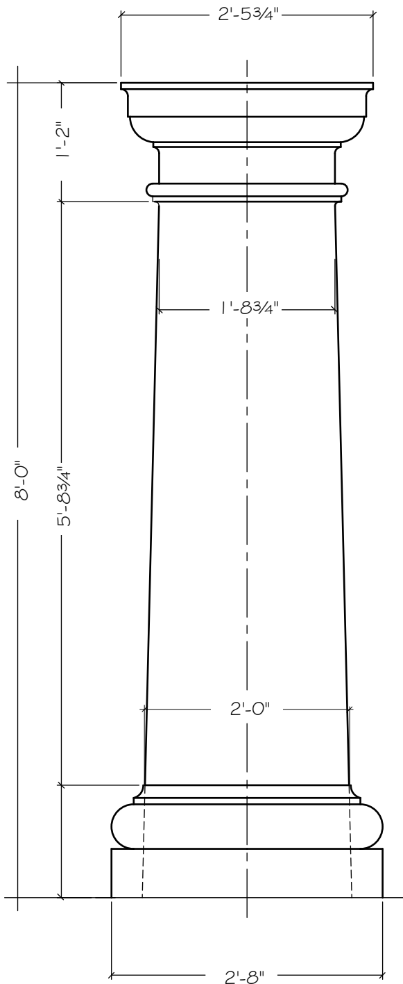
ELEVATION OF EC-120D COLUMN COVER
