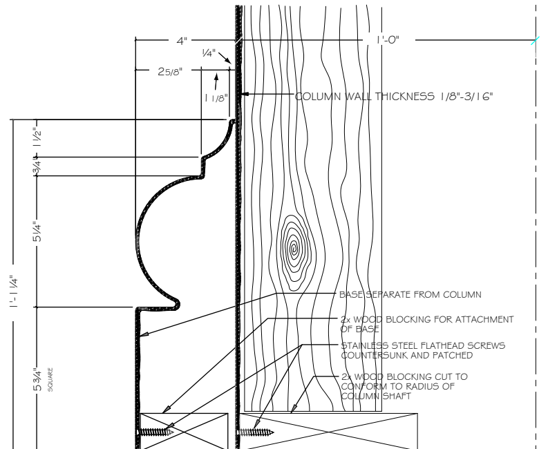
SECTION @ COLUMN BASE
