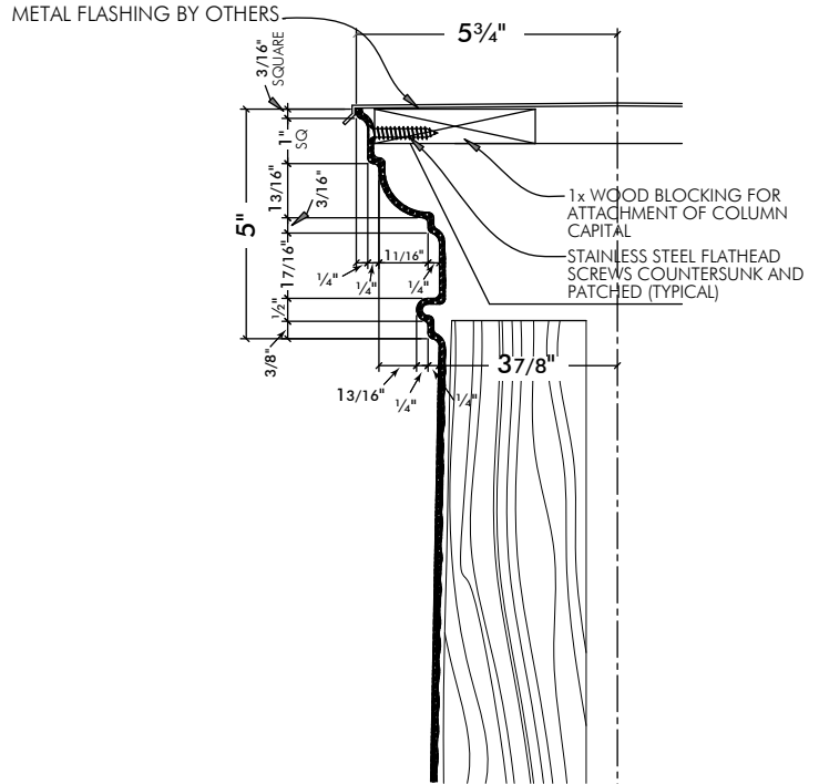
SECTION @ COLUMN CAPITAL
