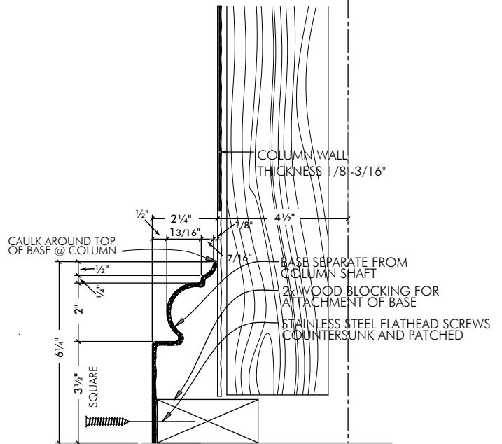
SECTION @ COLUMN BASE
