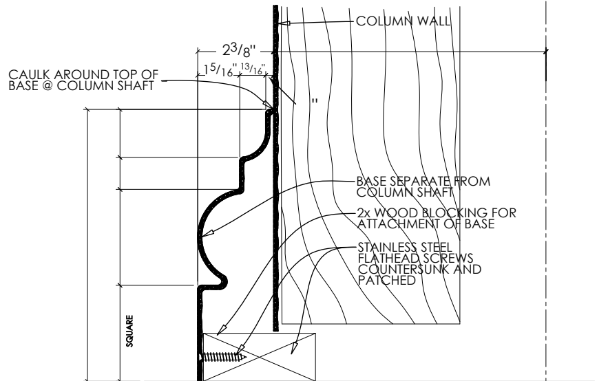
SECTION @ COLUMN BASE
