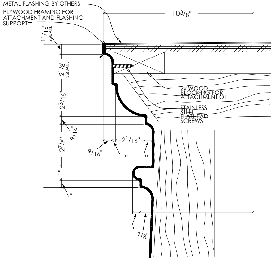
SECTION @ COLUMN CAPITAL
