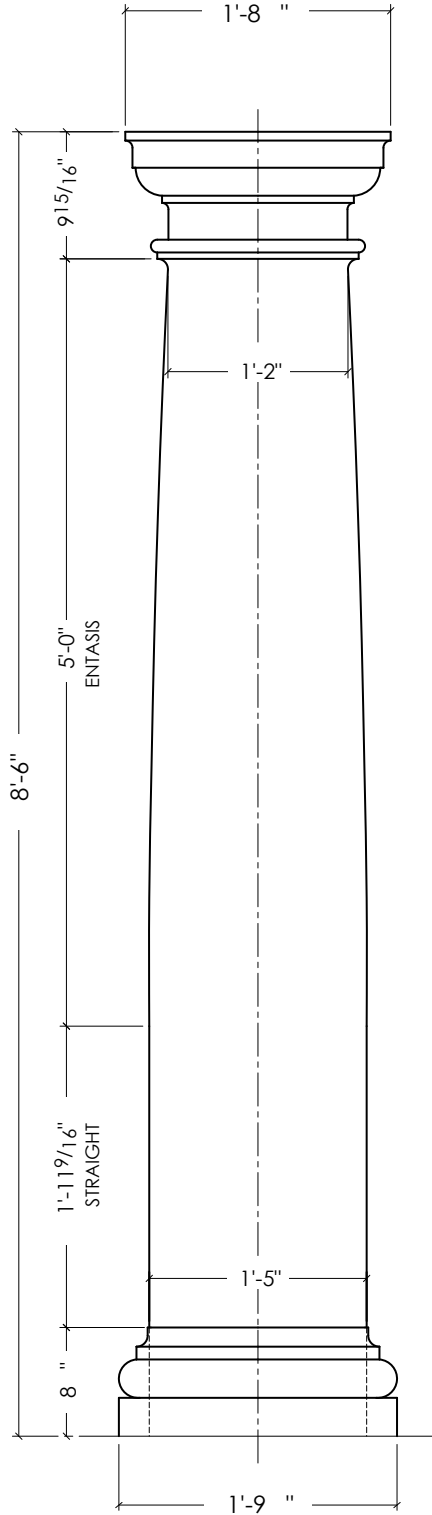
ELEVATION OF EC-120J.1 COLUMN COVER
