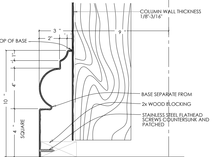
SECTION @ COLUMN BASE
