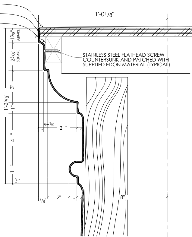
SECTION @ COLUMN CAPITAL
