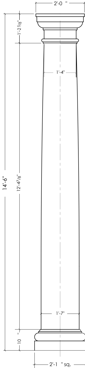
ELEVATION OF EC-120L COLUMN COVER
