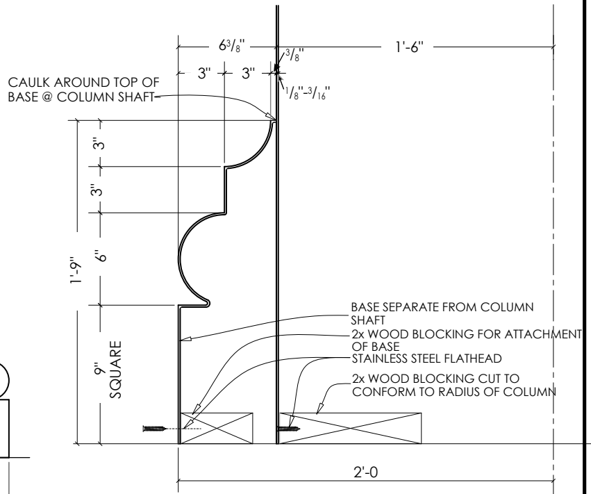
SECTION @ BASE
