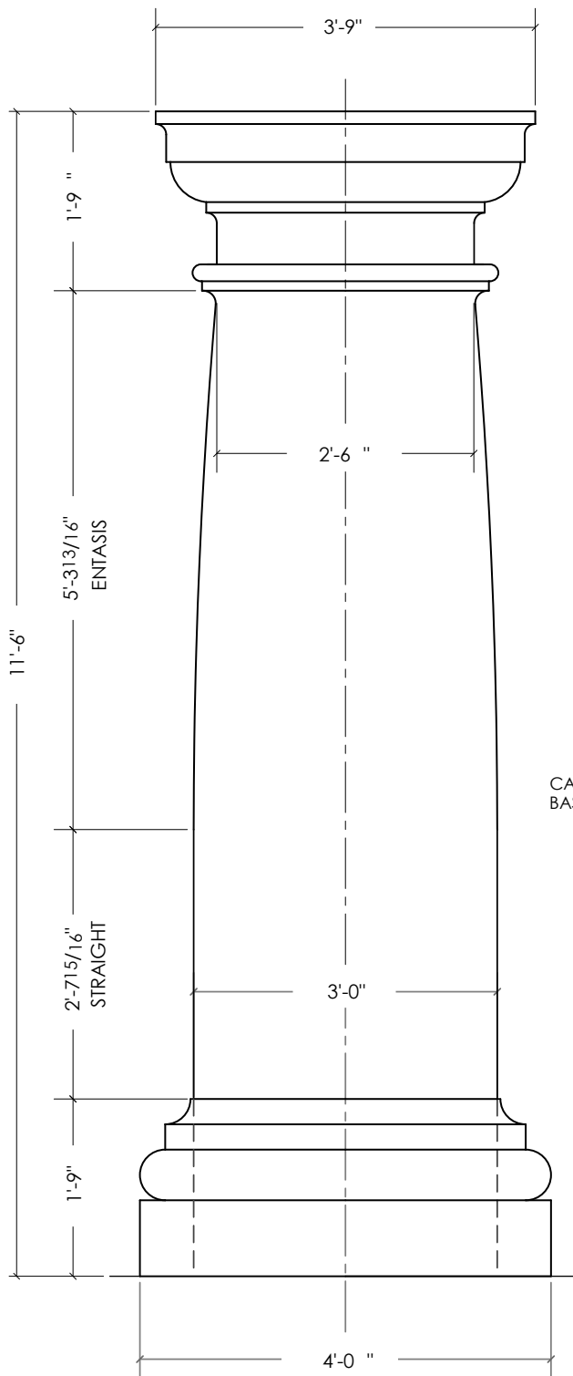
ELEV. of EC-120Q.1
