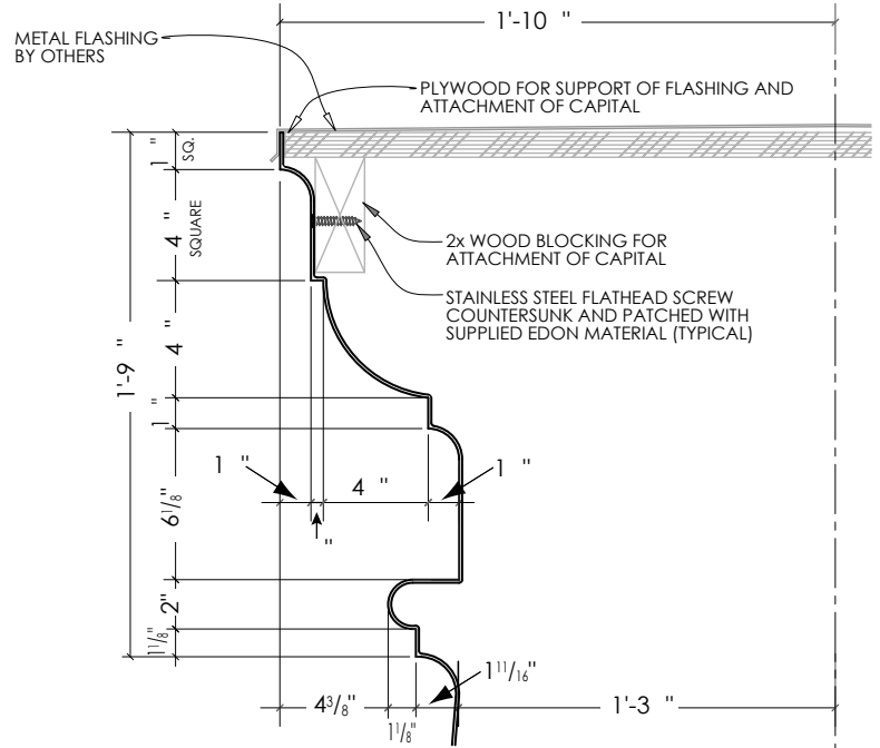
SECTION @ COLUMN CAPITAL
