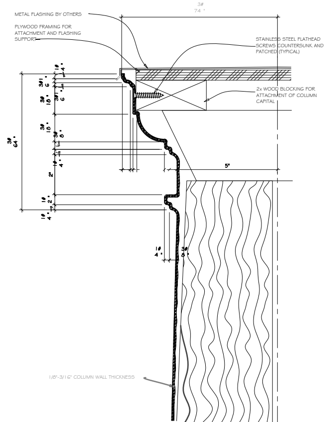
SECTION @ COLUMN CAPITAL
