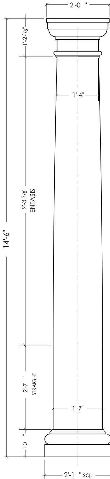
ELEVATION OF EC-120S COLUMN COVER
