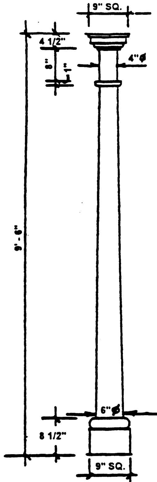
EC-120W 6" DIA. TAPERED TUSCAN COLUMN COVER
