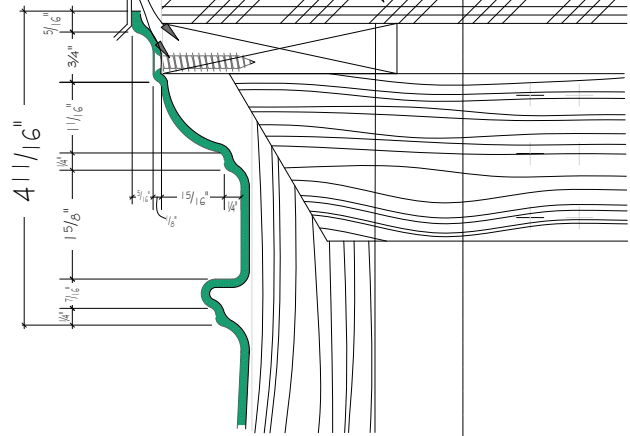
SECTION @ COLUMN CAPITAL
