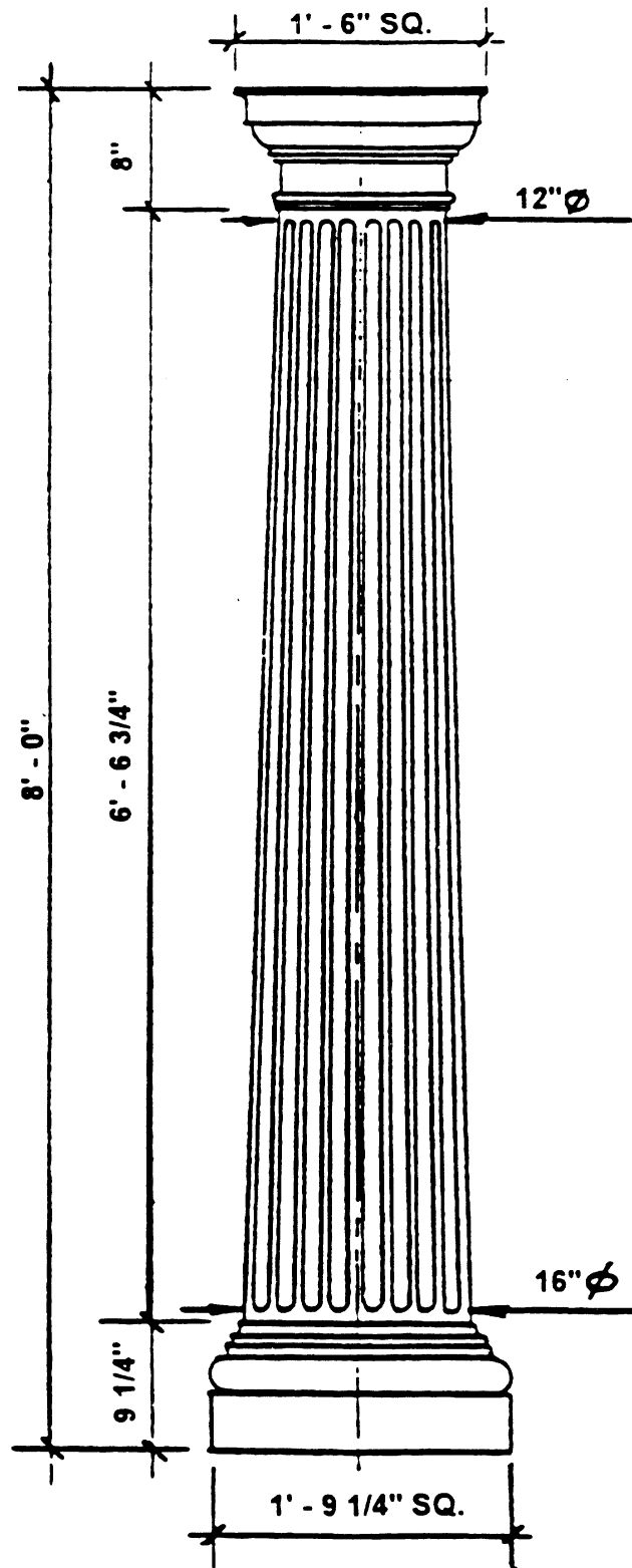
EC-141 8" DIA. FLUTED TAPERED SHAFT COLUMN
