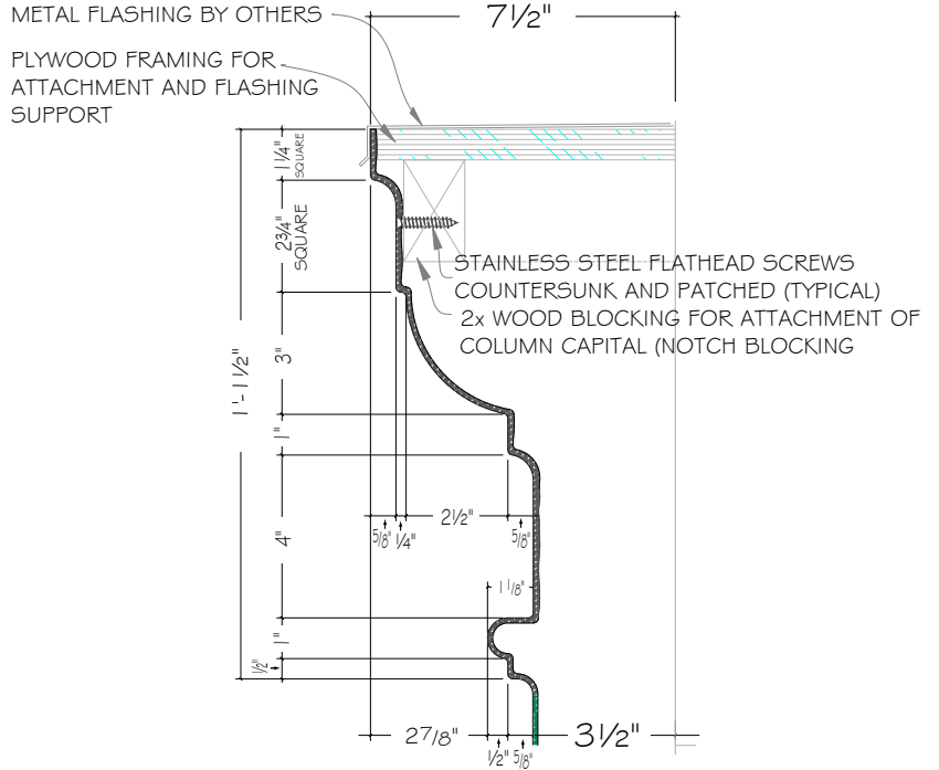
SECTION @ PILASTER CAPITAL
