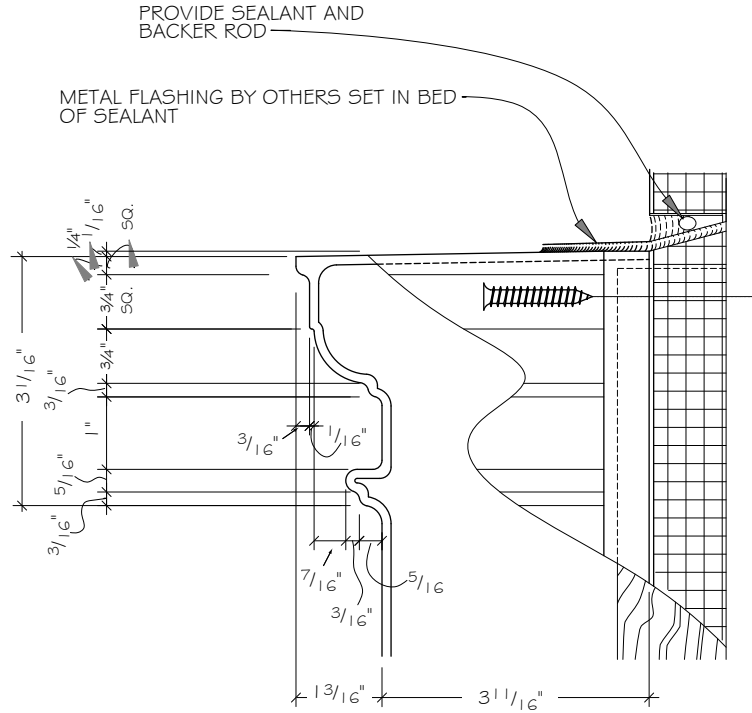
SECTION @ PILASTER CAPITAL
